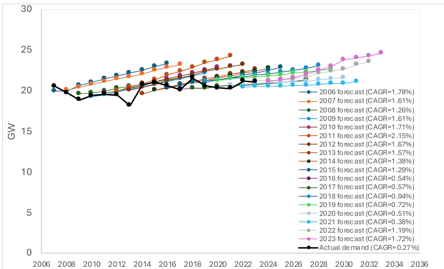
FIGURE 3 DUKE ENERGY CAROLINAS' PEAK DEMAND FORECASTS
